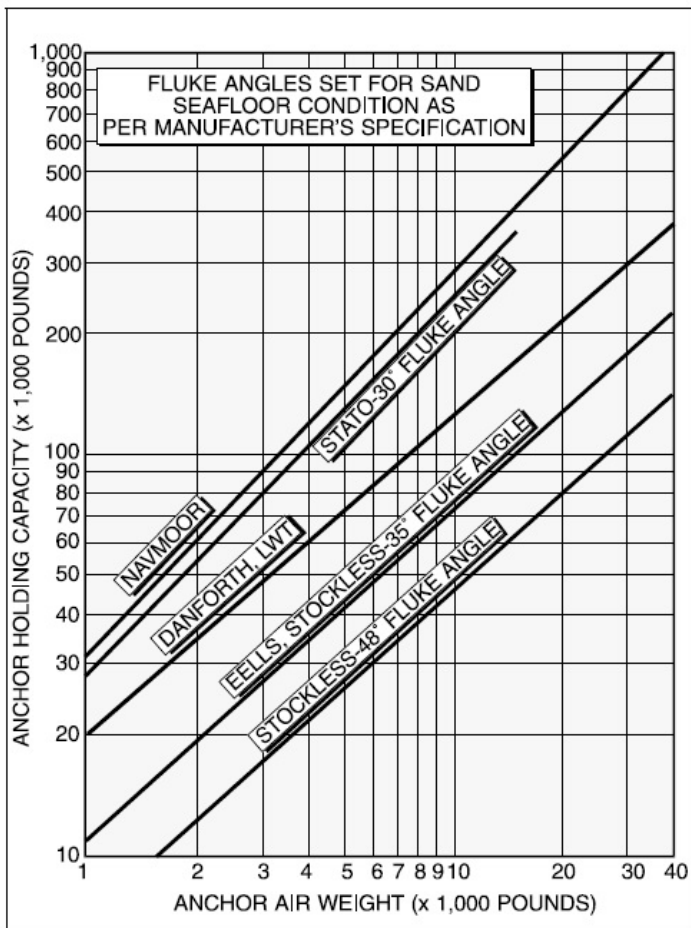
Figure 3-10. Drag Anchor System Holding Capacity in Sand.
