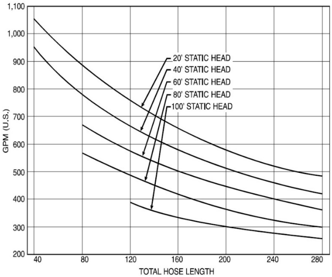
Figure 7-4M. Performance Curve, (Warm #6) CCN-150 Pump (6" Hose).
