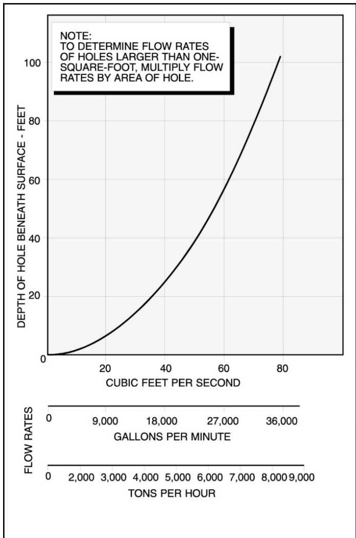
Figure 1-2. Flow Through a One-Square-Foot Hole.
