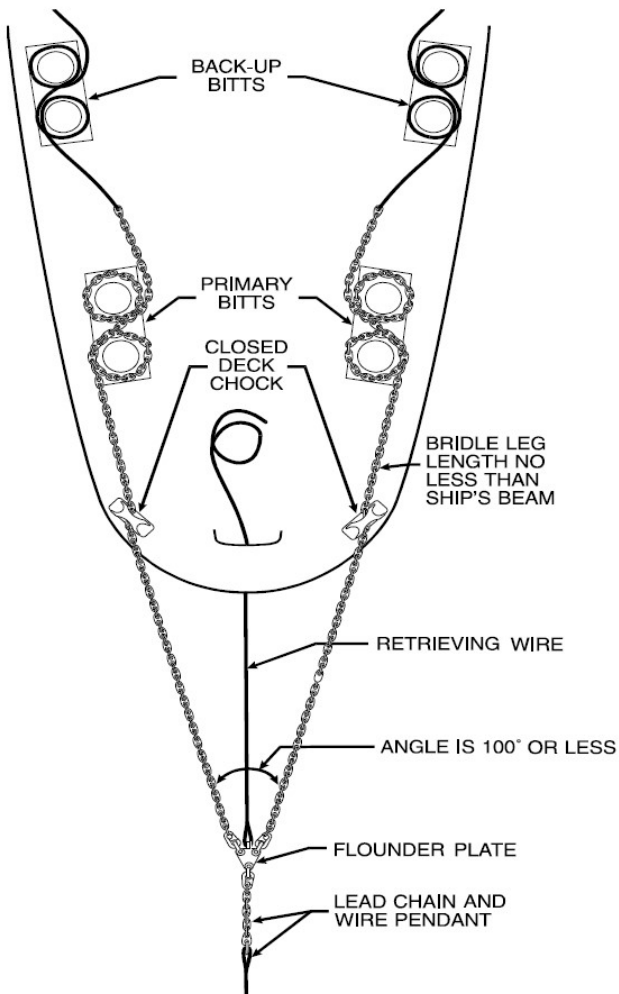
Figure 6-6A. Chain Bridle or Double Rig.
