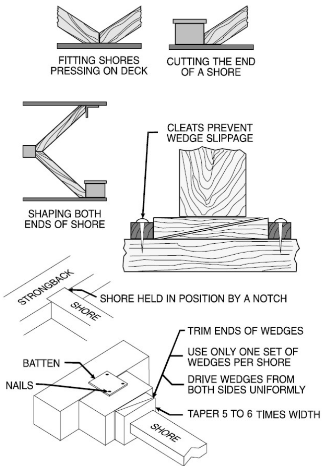
Figure 5-14. Anchoring Shores.
