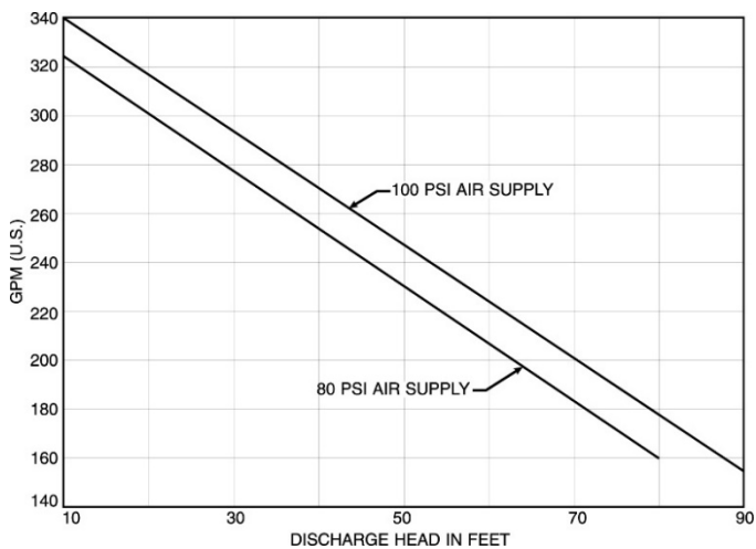
Figure 7-4D. Performance Curve, 2 1/2" Air Submersible Pump.
