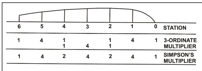
Figure 2-11. Simpson's Multipliers for Long Curve.
