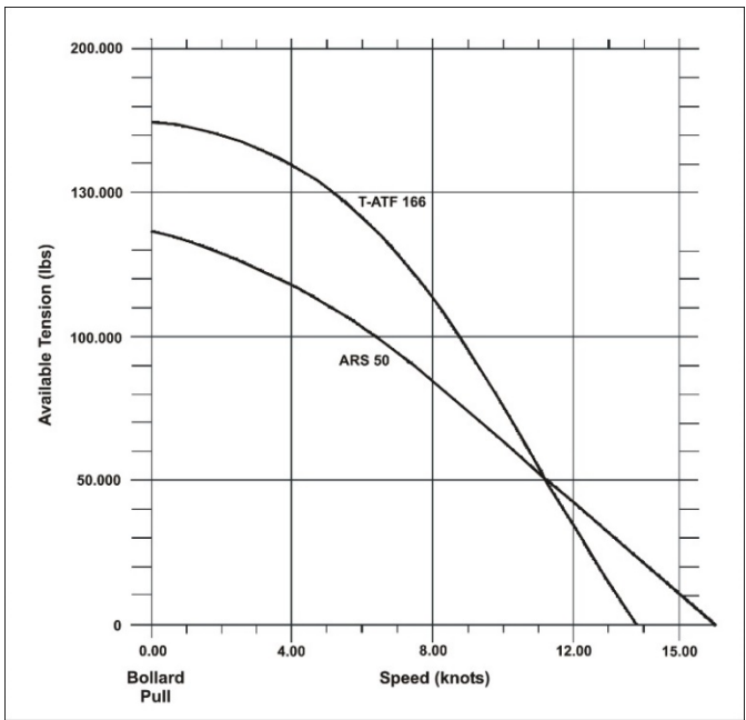
Figure 7-7. Available Tension vs. Ship's Speed for U.S. Navy Towing Ships.
