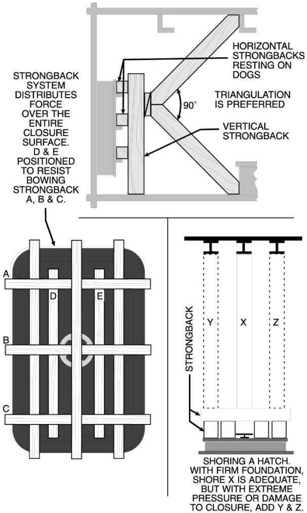
Figure 5-16. Shoring Doors and Hatches.
