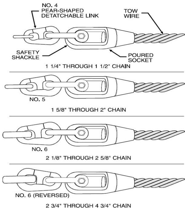
Figure 6-7. Towline Connections.
