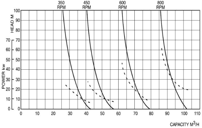
Figure 7-4P. Performance Curve, (Water) DOP-250 Pump.
