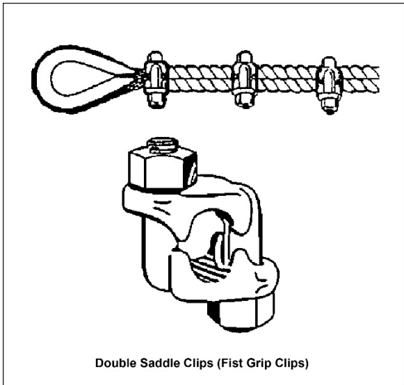
Figure 3-4. Double Saddle Clips (Fist Grip Clips).
