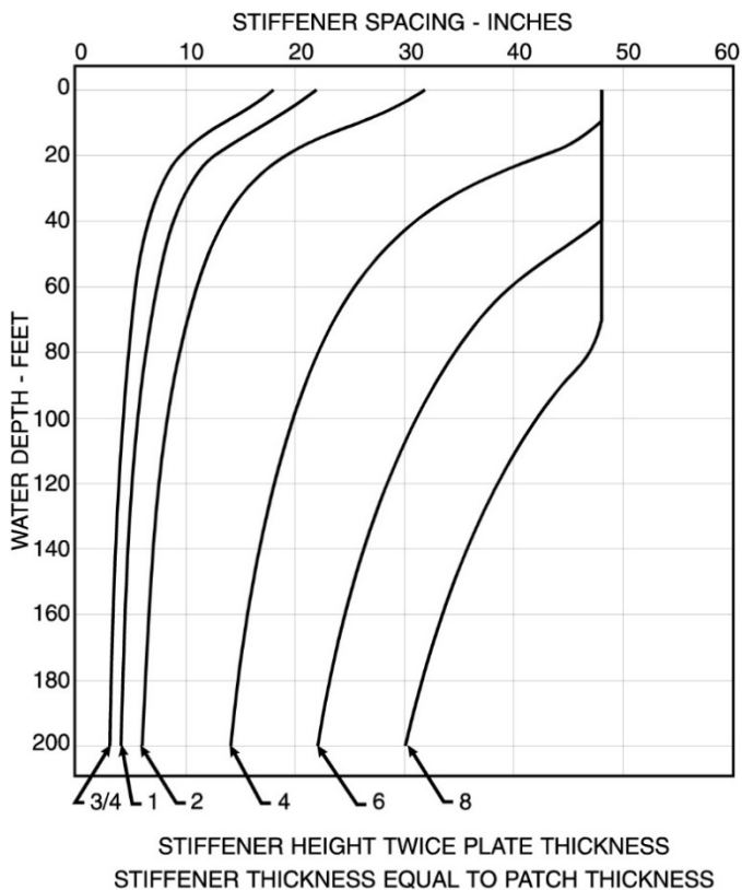
Figure 5-2B. Word Patch Stiffener Spacing.
