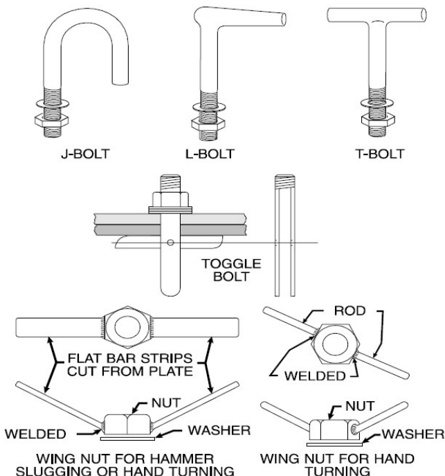
Figure 5-6. Patch Fasteners.
