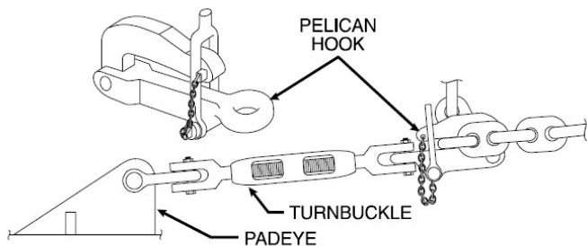
Figure 6-2. Chain Stopper.
