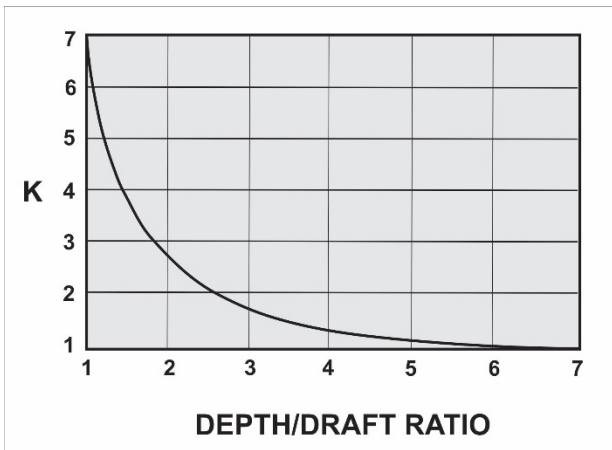
Figure 7-4R. Current Force Depth Correction Factor (K)
