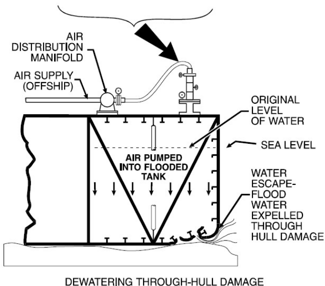
Figure 5-20A. Blowing Techniques.
