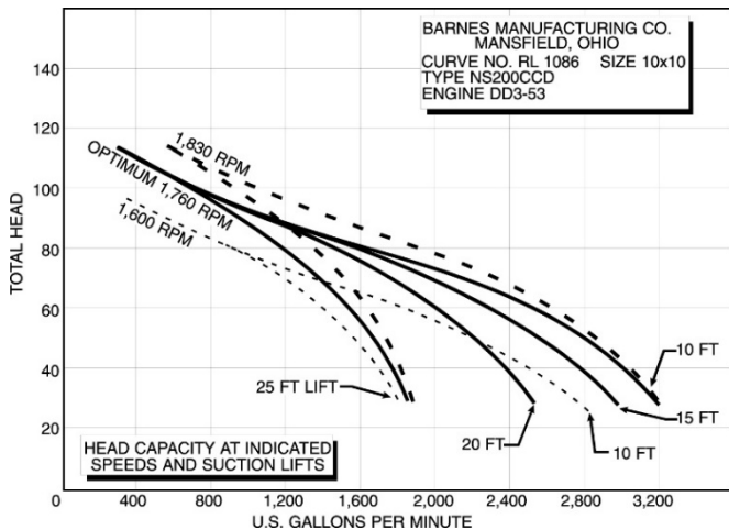
Figure 7-4C. Performance Curve, 10" Diesel Pump.
