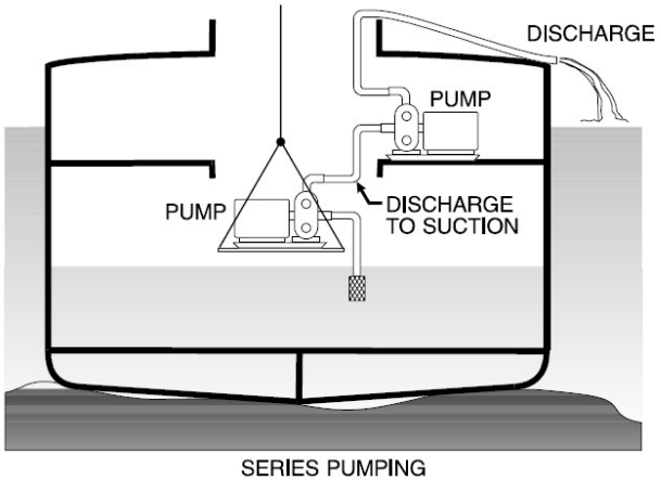
Figure 5-19A. Pumping Arrangements.
