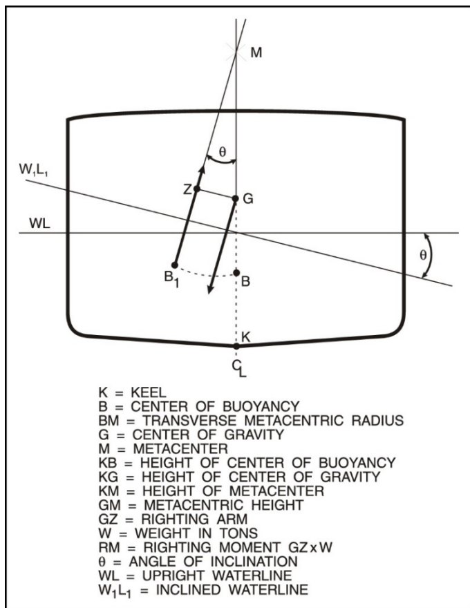
Figure 2-1. Centers, Heights and Righting Arm.
