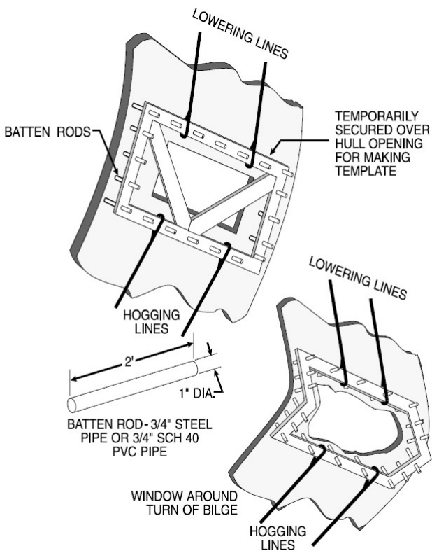
Figure 5-5. Hole Measuring Techniques and Device.
