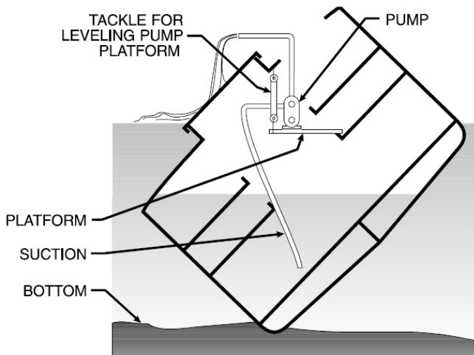
Figure 5-19C. Pumping Arrangements.
