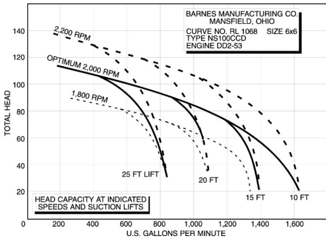
Figure 7-4B. Performance Curve, 6-inch Diesel Pump.
