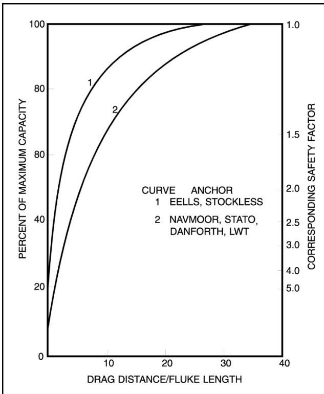
Figure 3-11. Anchor Holding Capacity versus Drag Distance in Mud.
