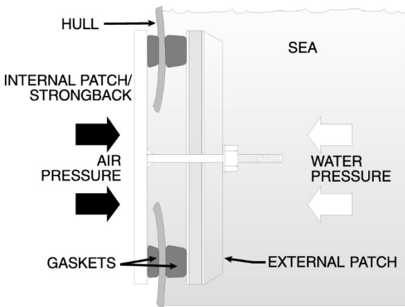
Figure 5-1. Double Patch.
