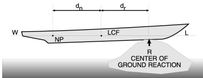
Figure 4-1. Distances Needed to Locate the Neutral Loading Point.
