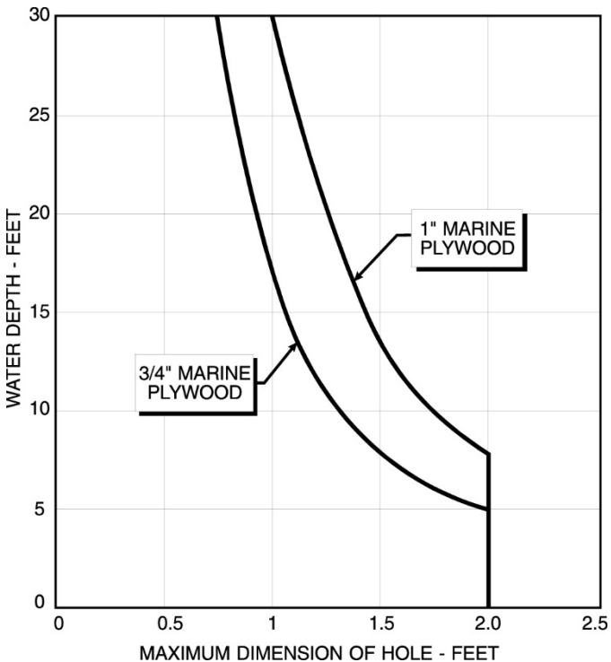
Figure 5-3. Plywood Patch Thickness
