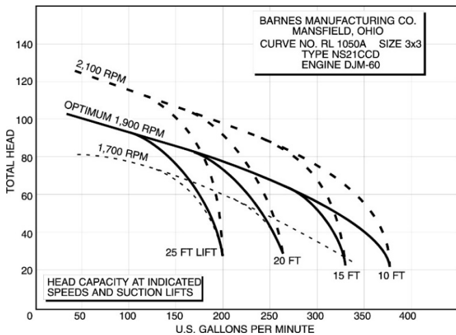
Figure 7-4A. Performance Curve, 3" Diesel Pump.
