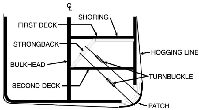
Figure 5-8. Patch Secured with Turnbuckle and Strongback.
