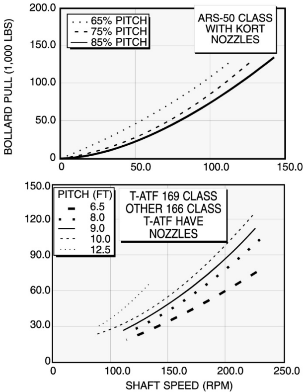
Figure 7-5. Bollard Pull Curves
