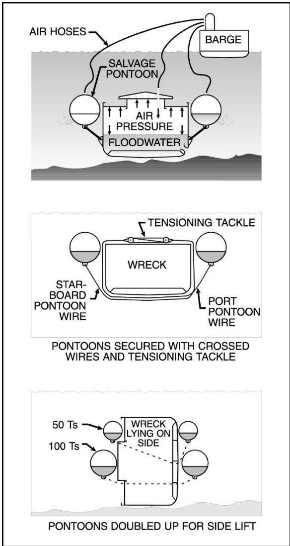
Figure 3-13. Rigging Pontoons and Lift Bags.
