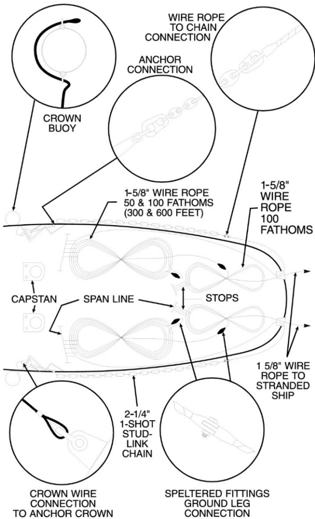
Figure 4-6. Rigging to Lay Ground Legs Seaward from Stranding.
