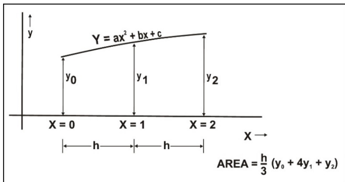
Figure 2-10. Simpson's Three-Ordinate Rule.
