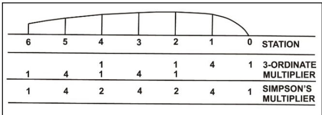
Figure 2-12. Simpson's Multipliers with Half-Space Stations.
