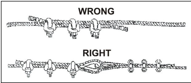
Figure 3-6. Joining Wire Ropes.
