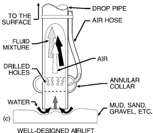
Figure 5-18. Air Lifts.
