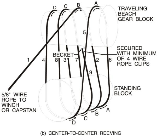
Figure 4-4 Reeving Blocks
