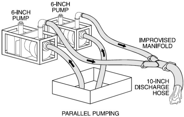
Figure 5-19B. Pumping Arrangements.
