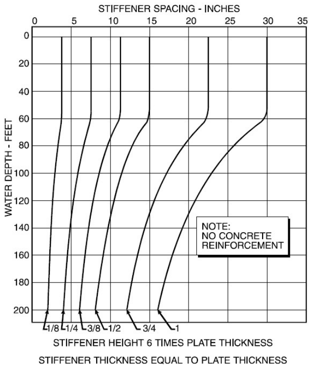
Figure 5-2A. Steel Patch Stiffener Spacing.
