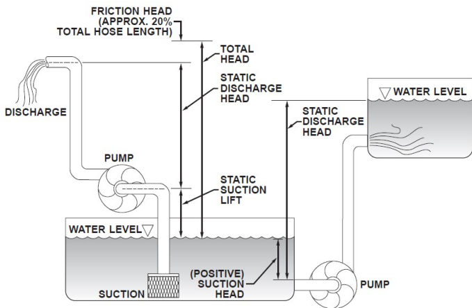
Figure 5-17. Pumping Heads.
