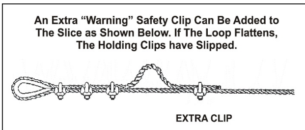
Figure 3-5. Joining Wire Ropes.
